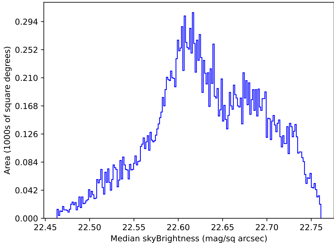
early_ss_template_fpextra2.0_v3.4_10yrs Yr 1 u band: Median skyBrightness
