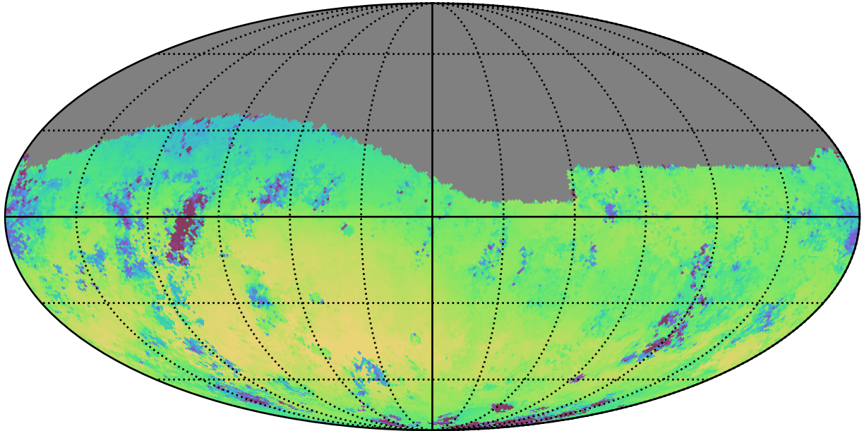
early_ss_template_fpextra2.0_v3.4_10yrs Yr 1 r band: Median skyBrightness
