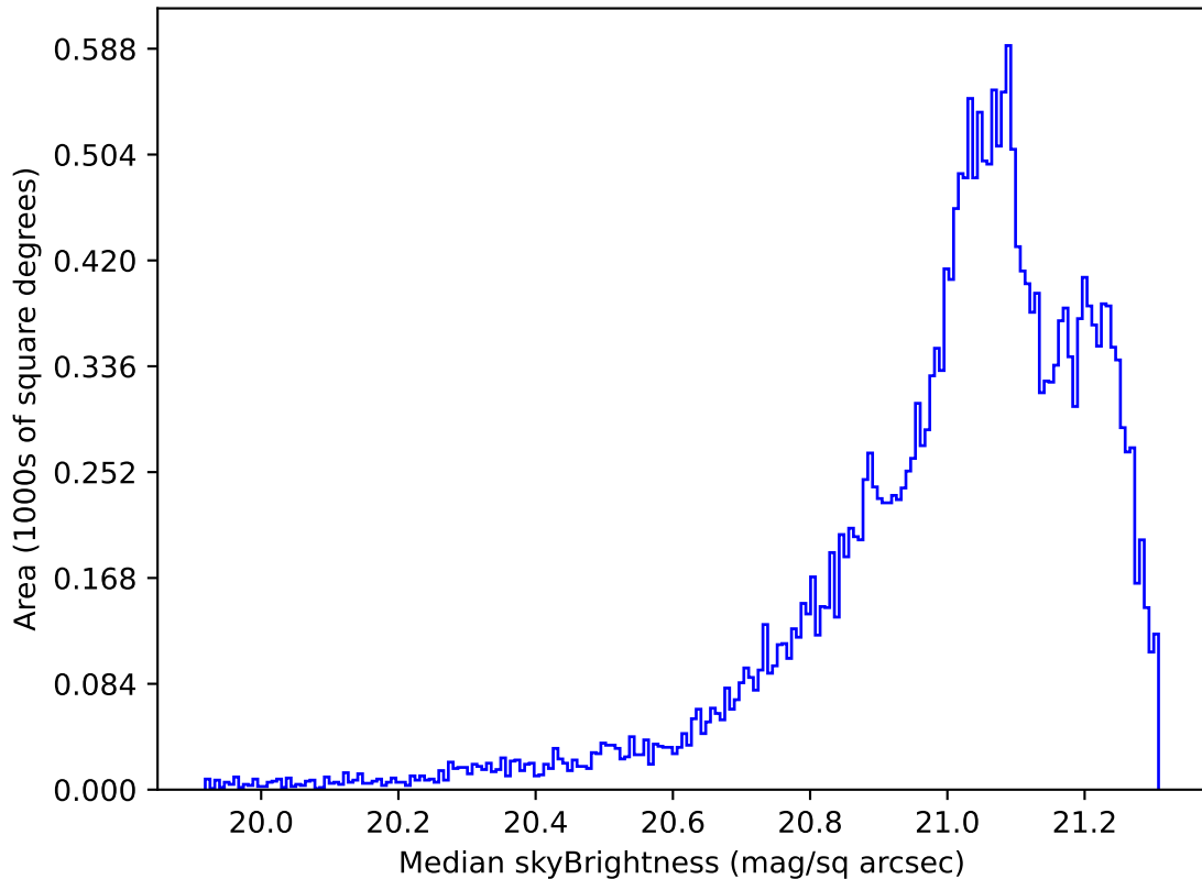
early_ss_template_fpextra2.0_v3.4_10yrs Yr 1 r band: Median skyBrightness
