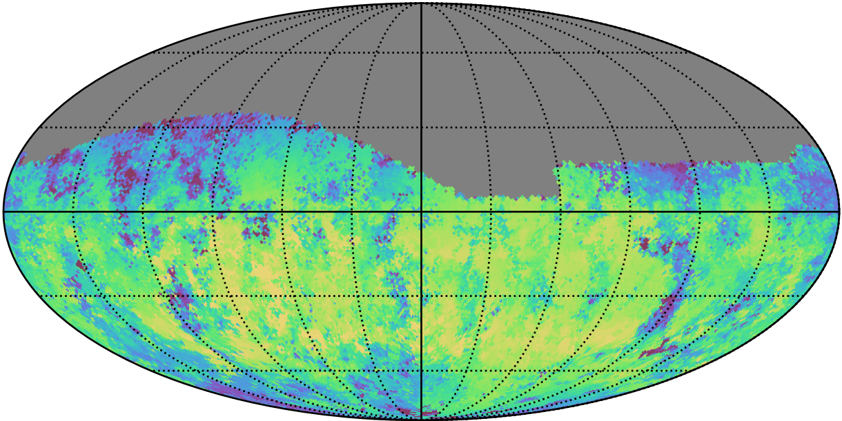
early_ss_template_fpextra2.0_v3.4_10yrs Yr 1 i band: Median skyBrightness
