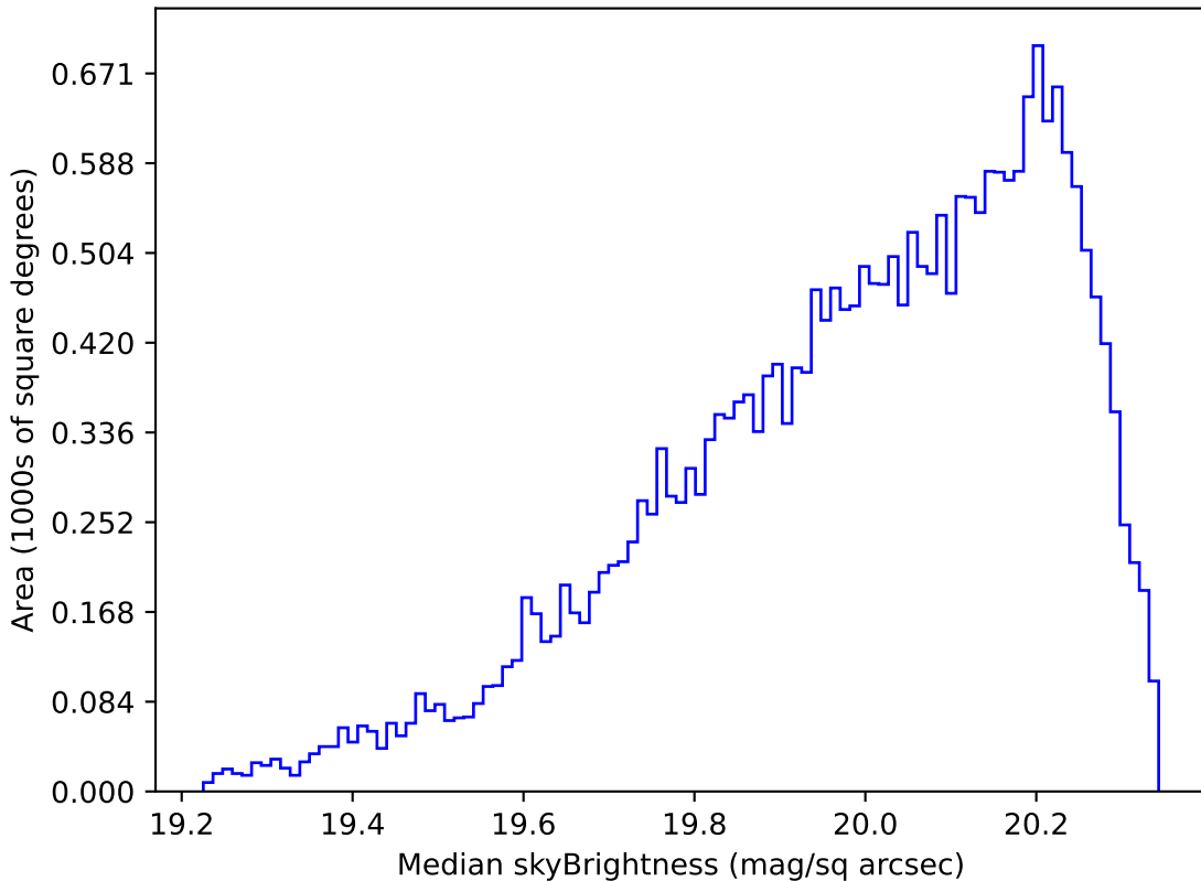
early_ss_template_fpextra2.0_v3.4_10yrs Yr 1 i band: Median skyBrightness
