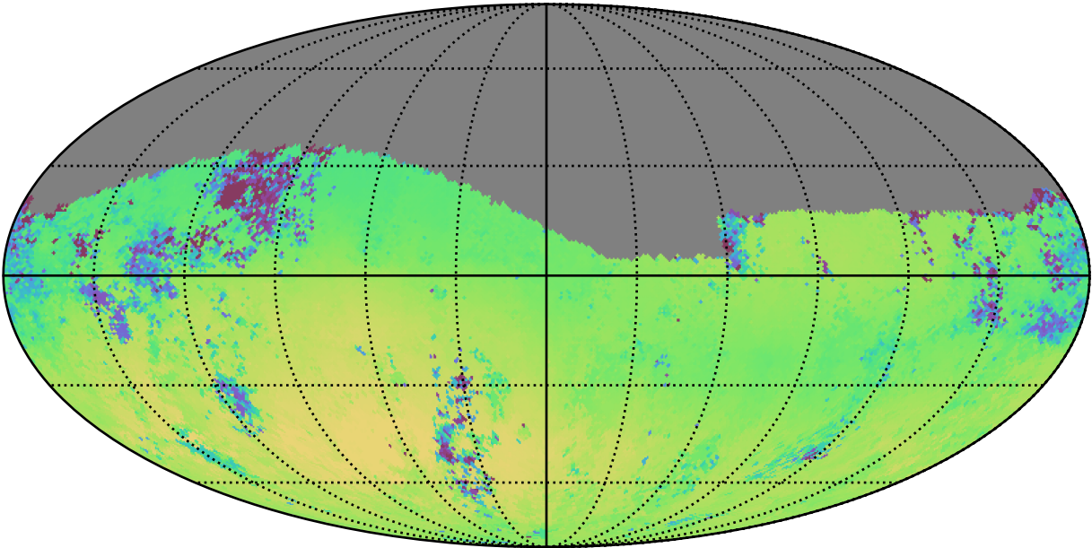
early_ss_template_fpextra2.0_v3.4_10yrs Yr 1 g band: Median skyBrightness
