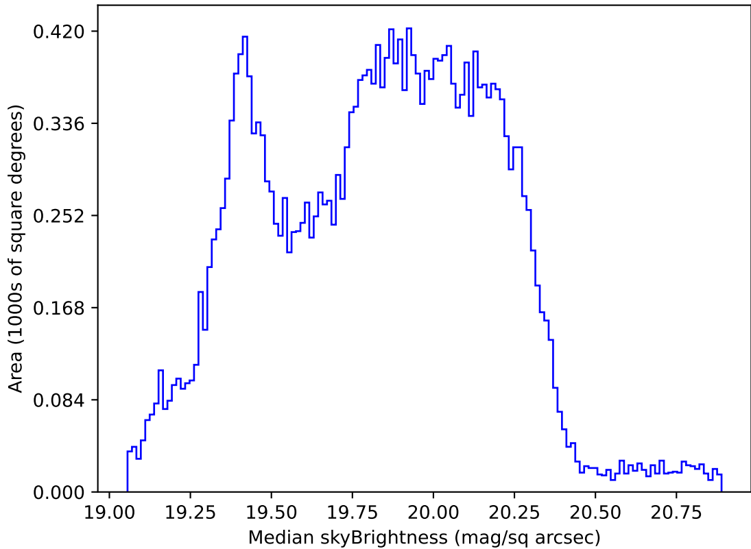
early_ss_template_fpextra2.0_v3.4_10yrs Yr 1 all bands: Median skyBrightness
