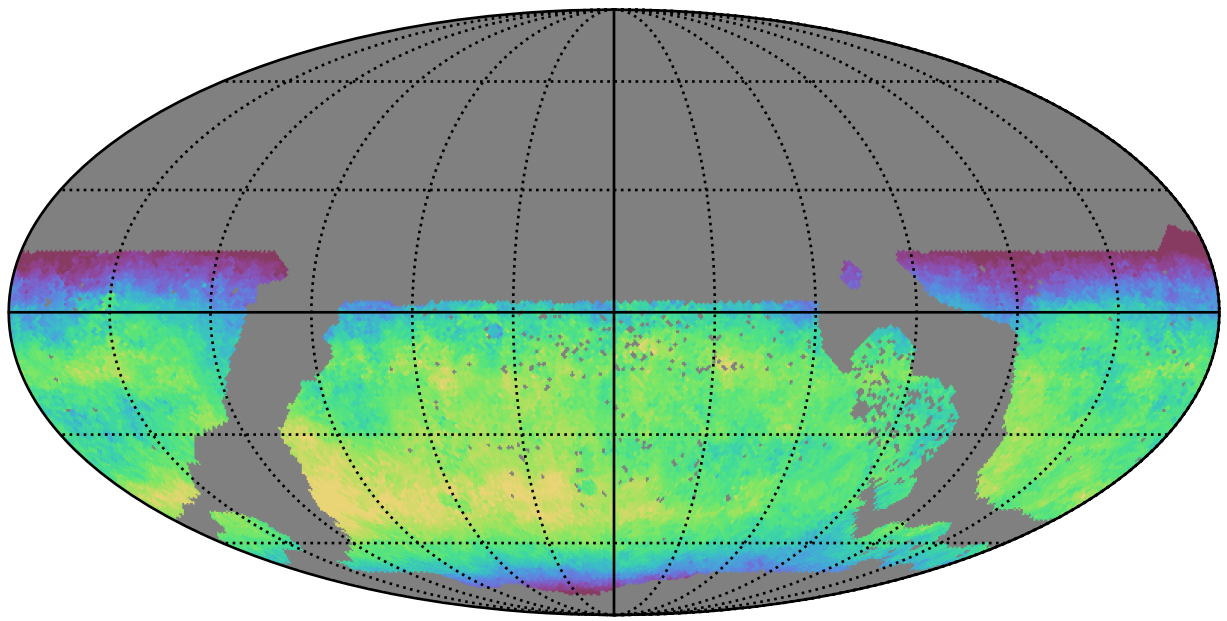
early_ss_template_fpextra2.0_v3.4_10yrs WFD y band: Median skyBrightness
