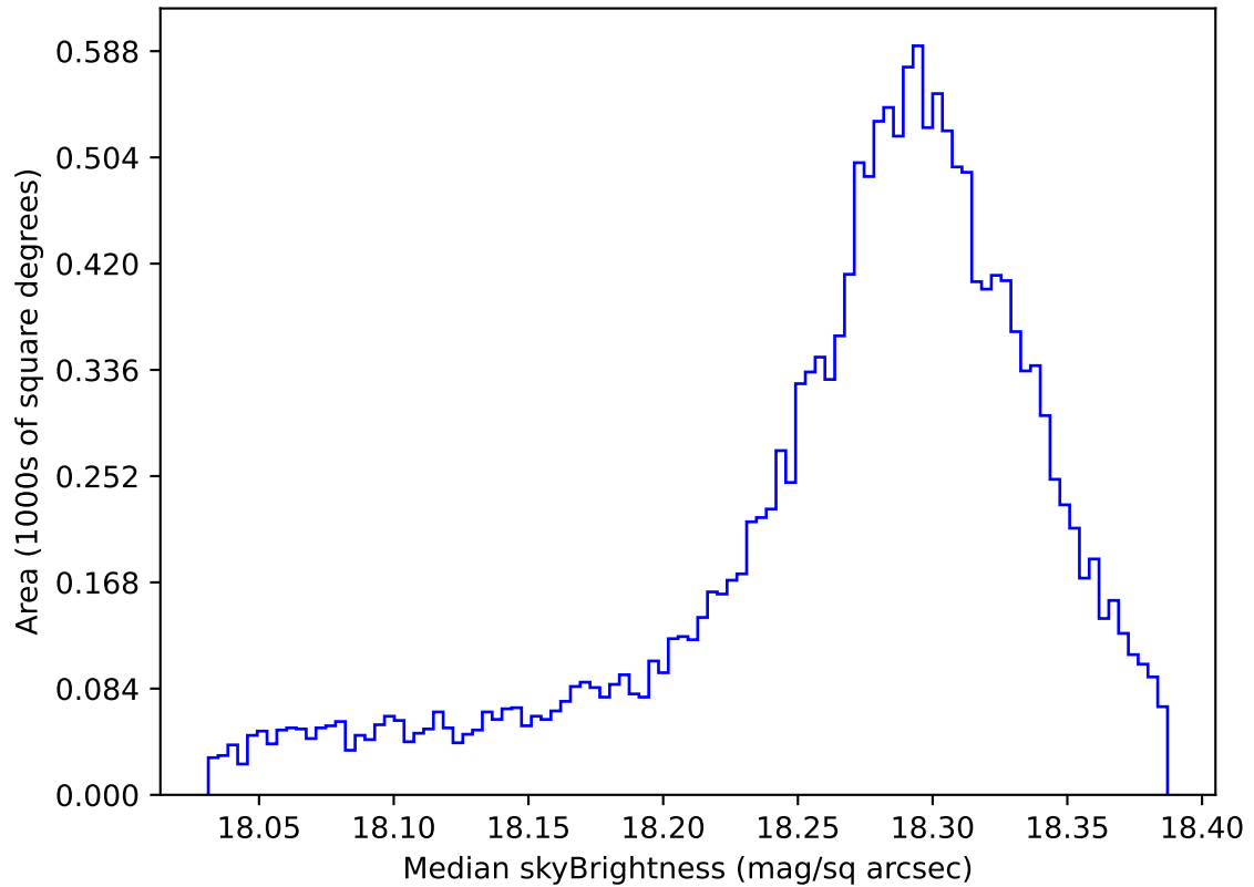
early_ss_template_fpextra2.0_v3.4_10yrs WFD y band: Median skyBrightness
