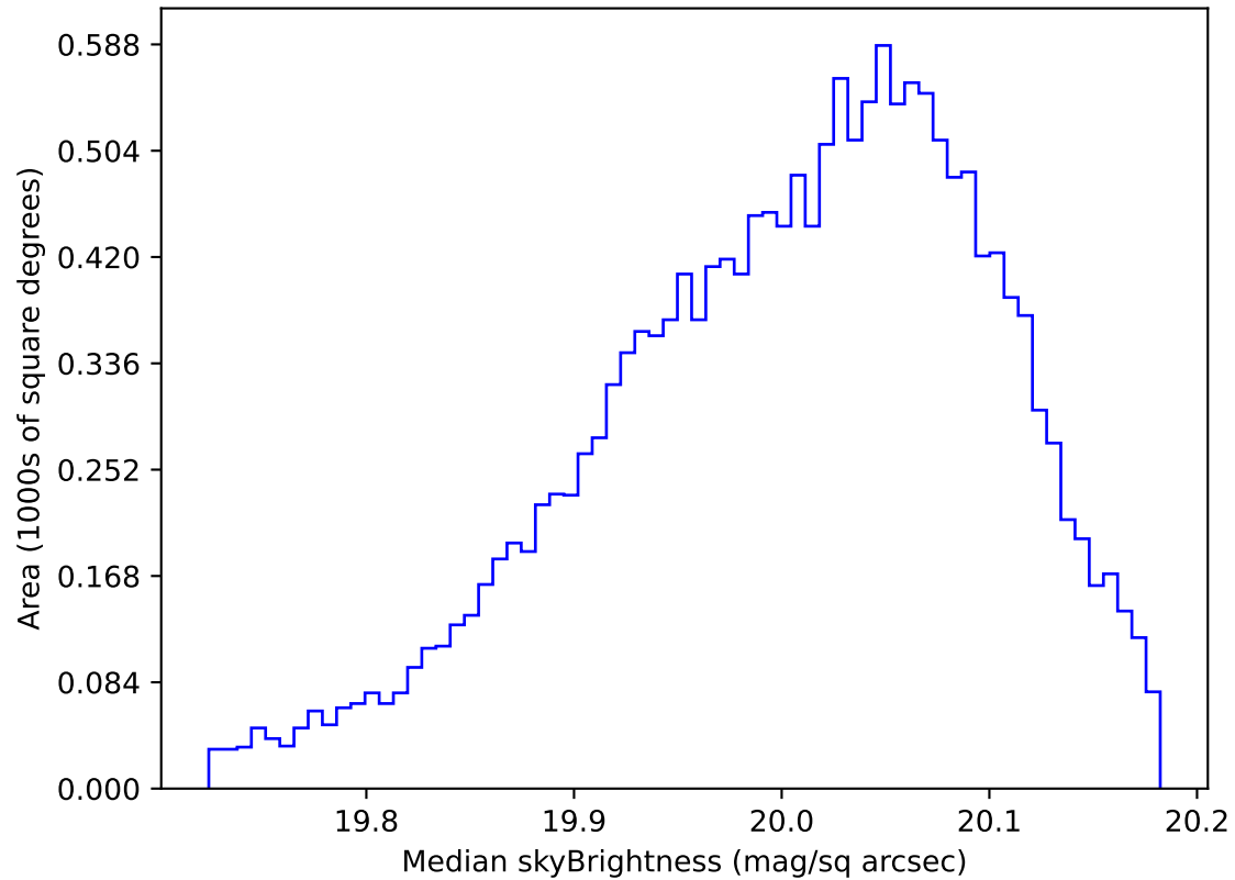
early_ss_template_fpextra2.0_v3.4_10yrs WFD i band: Median skyBrightness
