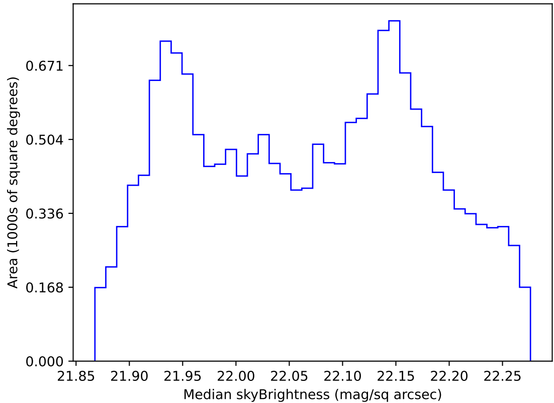
early_ss_template_fpextra2.0_v3.4_10yrs WFD g band: Median skyBrightness
