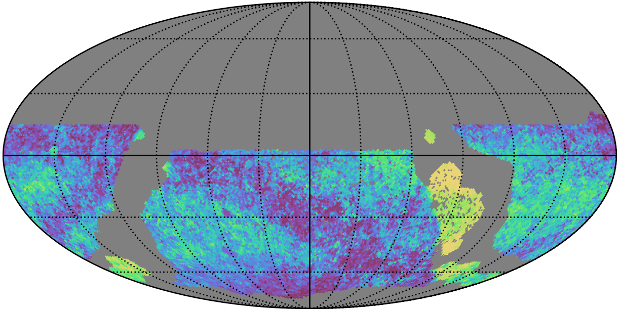
early_ss_template_fpextra2.0_v3.4_10yrs WFD all bands: Median skyBrightness
