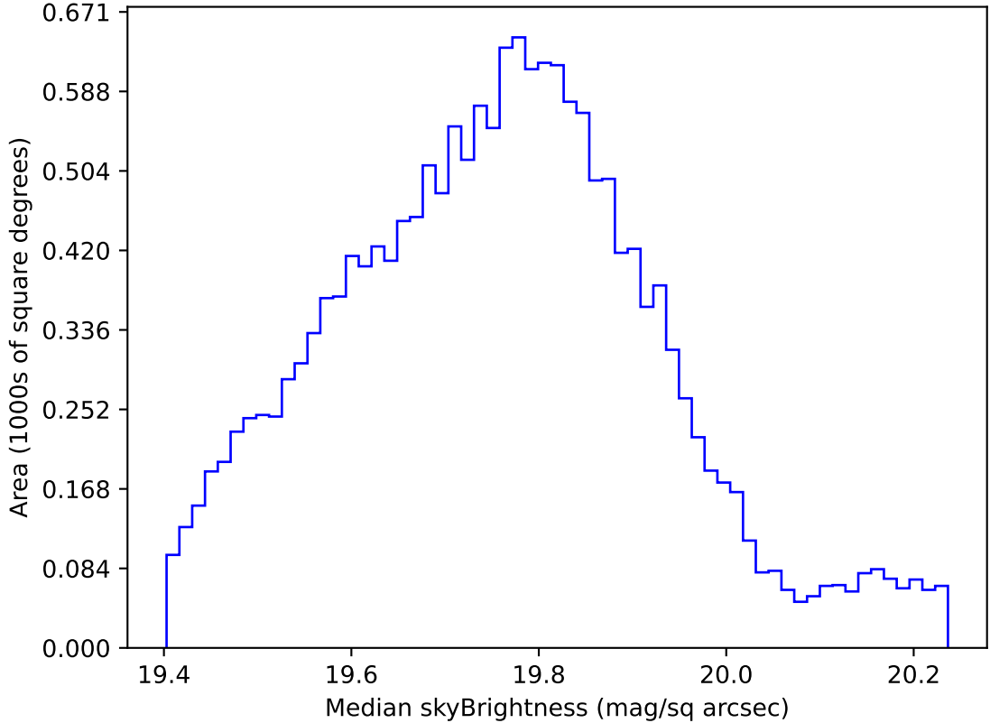
early_ss_template_fpextra2.0_v3.4_10yrs WFD all bands: Median skyBrightness
