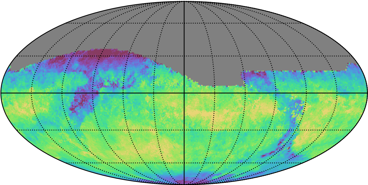
early_ss_template_fpextra2.0_v3.4_10yrs All sky z band: Median skyBrightness
