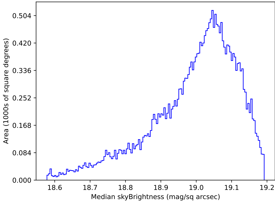
early_ss_template_fpextra2.0_v3.4_10yrs All sky z band: Median skyBrightness
