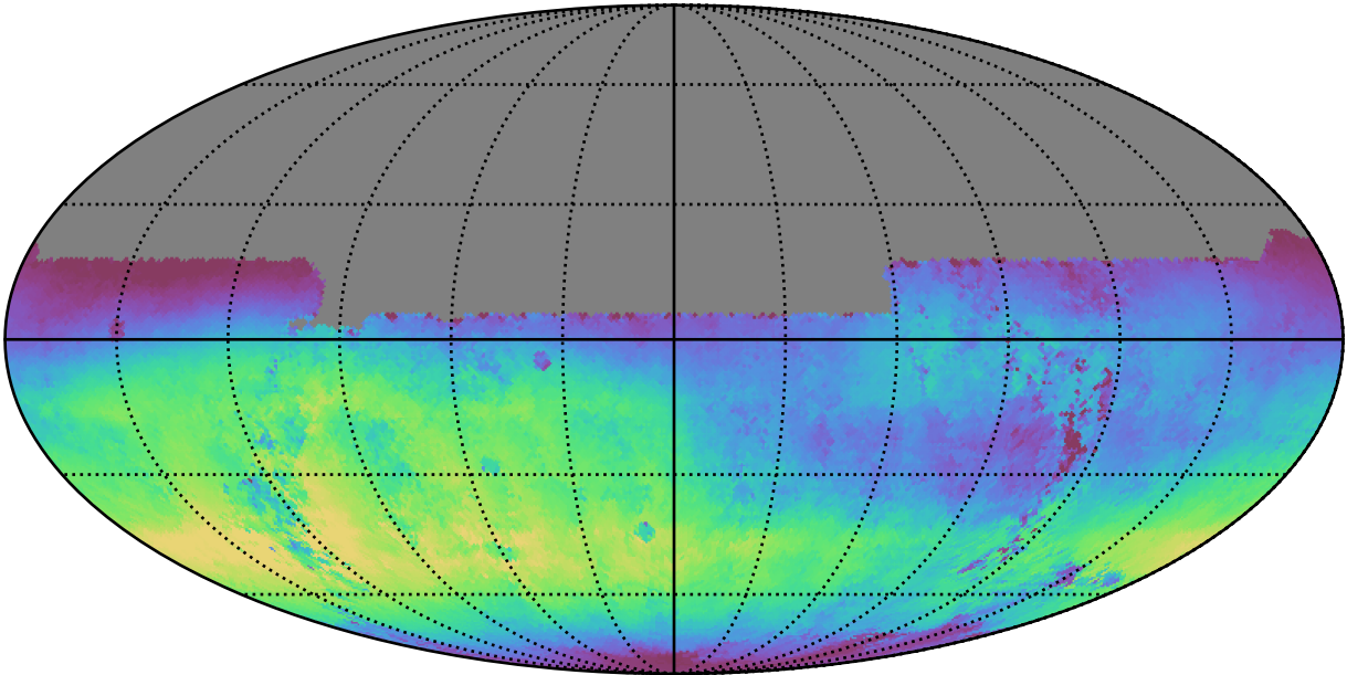
early_ss_template_fpextra2.0_v3.4_10yrs All sky u band: Median skyBrightness
