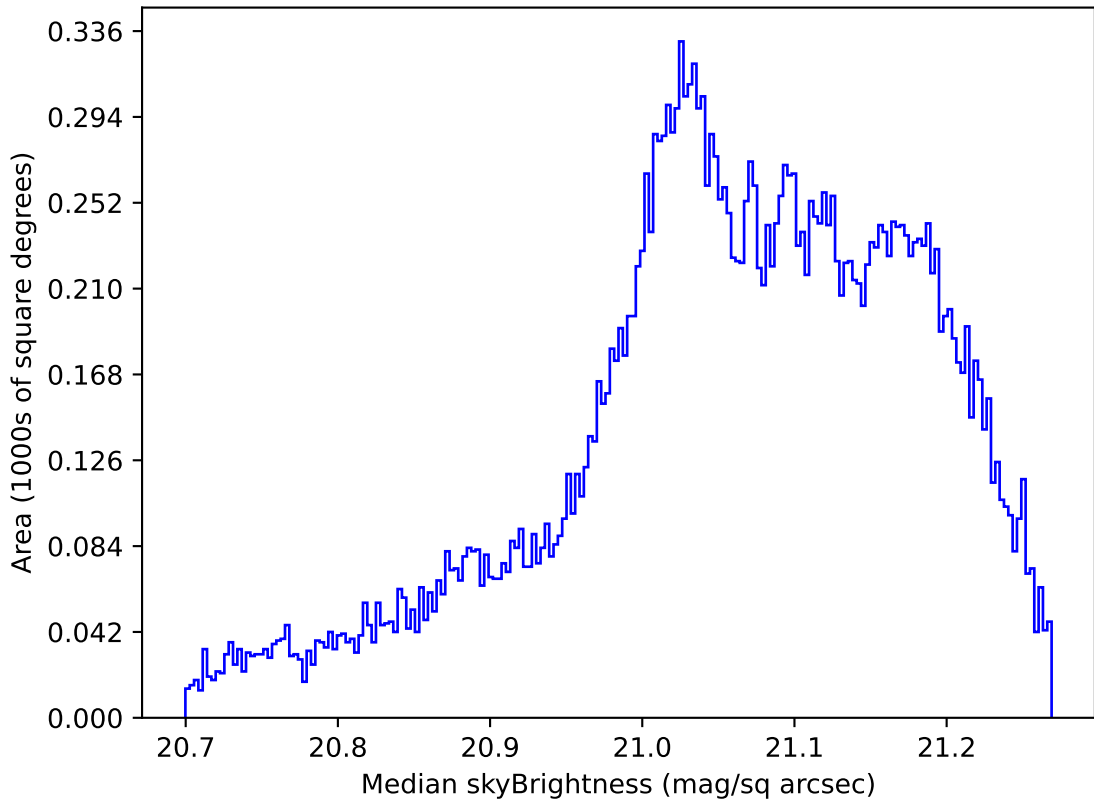
early_ss_template_fpextra2.0_v3.4_10yrs All sky r band: Median skyBrightness
