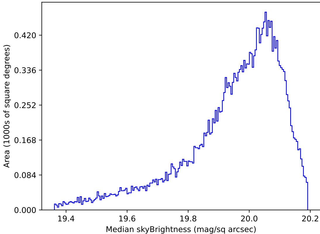
early_ss_template_fpextra2.0_v3.4_10yrs All sky i band: Median skyBrightness
