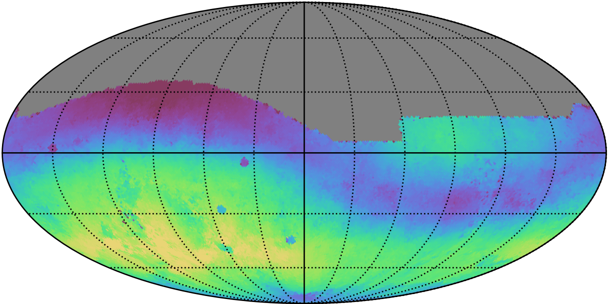
early_ss_template_fpextra2.0_v3.4_10yrs All sky g band: Median skyBrightness
