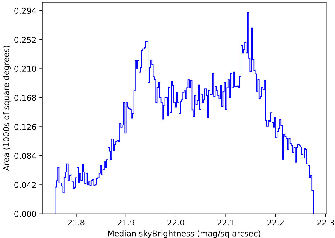
early_ss_template_fpextra2.0_v3.4_10yrs All sky g band: Median skyBrightness
