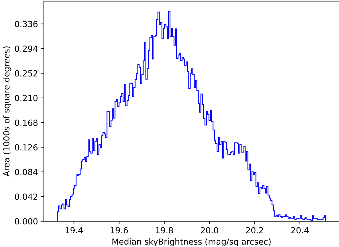
early_ss_template_fpextra2.0_v3.4_10yrs All sky all bands: Median skyBrightness
