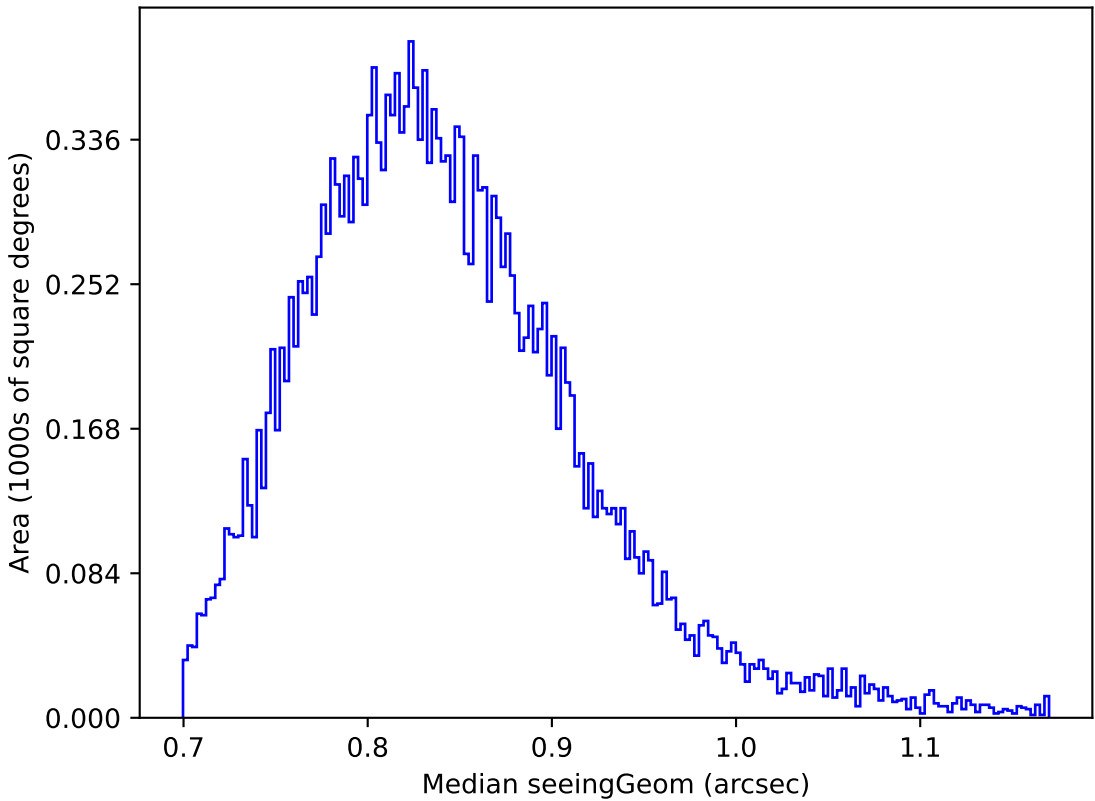
early_ss_template_fpextra2.0_v3.4_10yrs Yr 1 y band: Median seeingGeom
