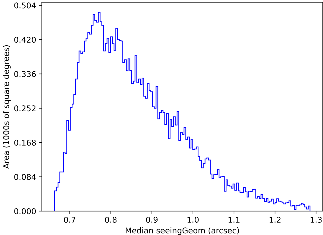
early_ss_template_fpextra2.0_v3.4_10yrs Yr 1 r band: Median seeingGeom
