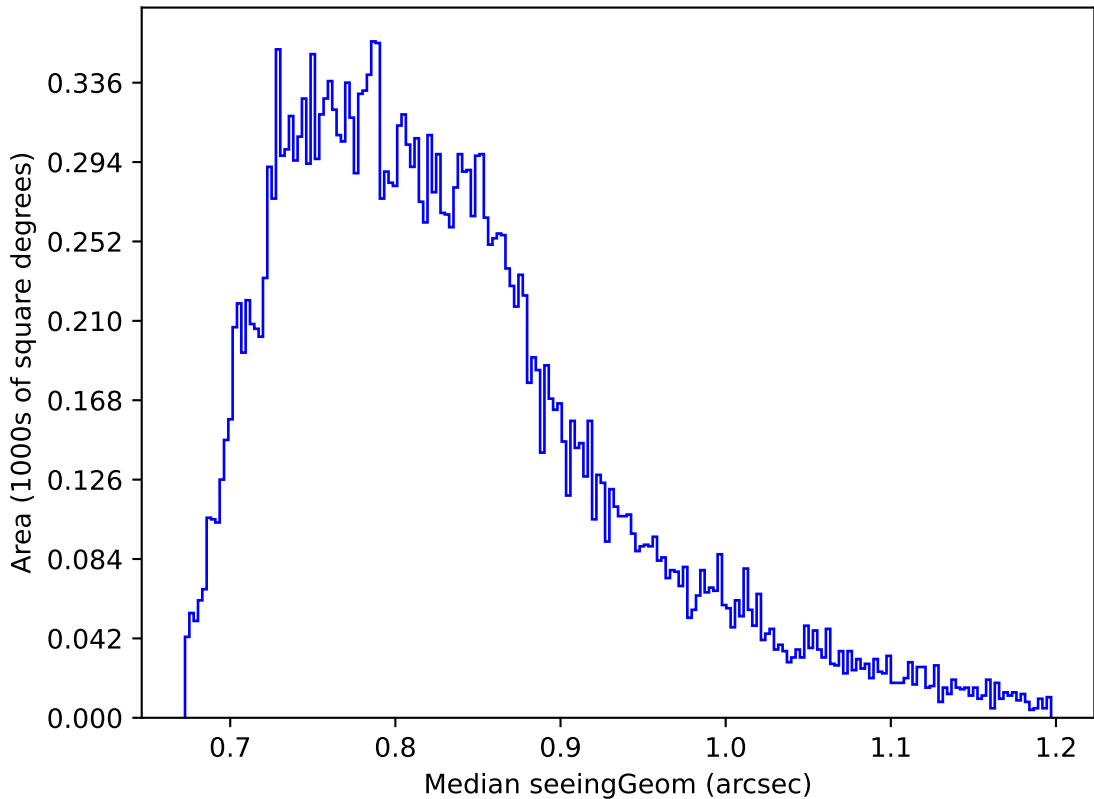
early_ss_template_fpextra2.0_v3.4_10yrs Yr 1 i band: Median seeingGeom
