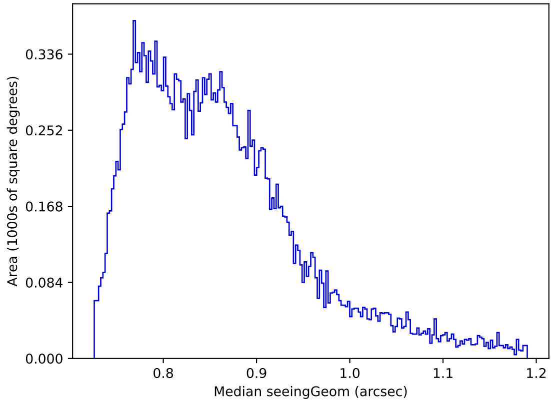
early_ss_template_fpextra2.0_v3.4_10yrs Yr 1 all bands: Median seeingGeom
