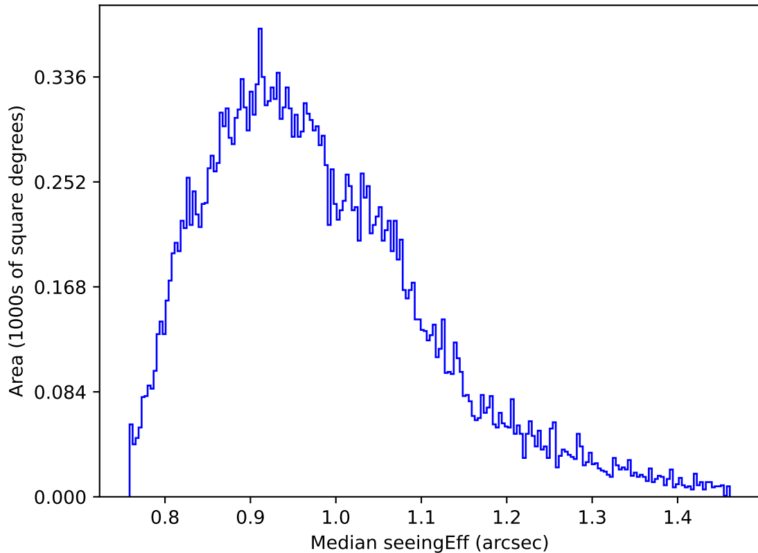
early_ss_template_fpextra2.0_v3.4_10yrs Yr 1 z band: Median seeingEff
