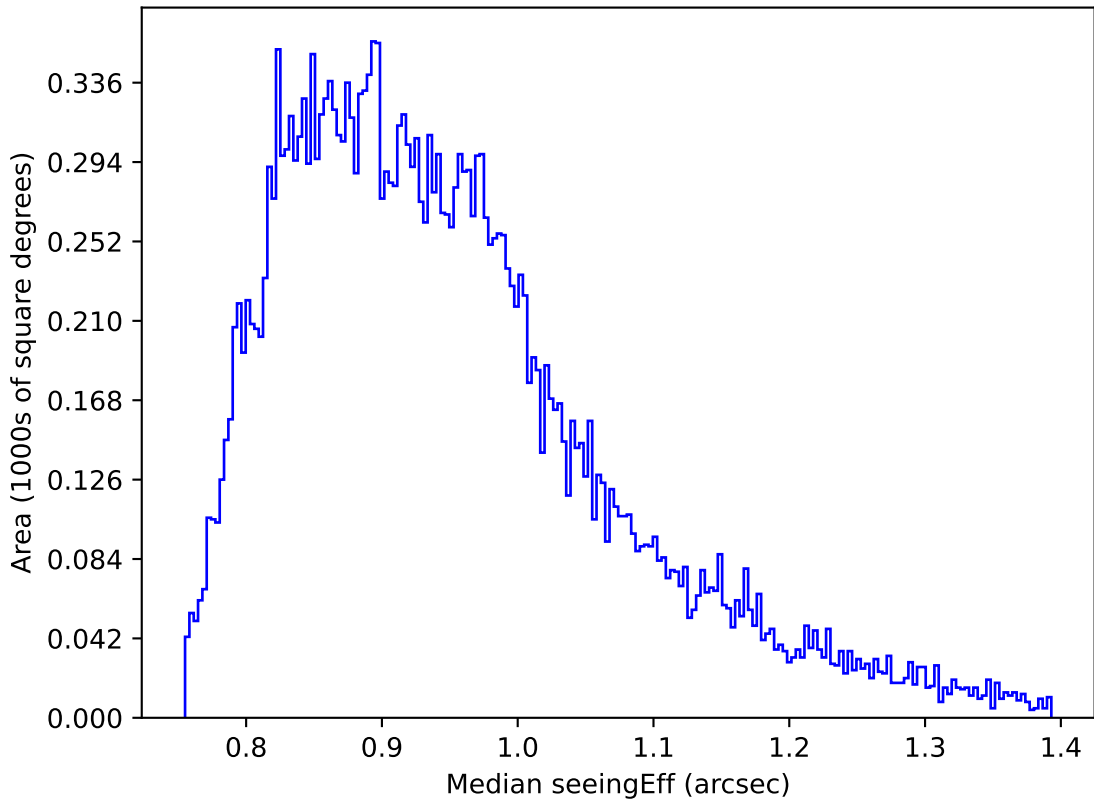
early_ss_template_fpextra2.0_v3.4_10yrs Yr 1 i band: Median seeingEff
