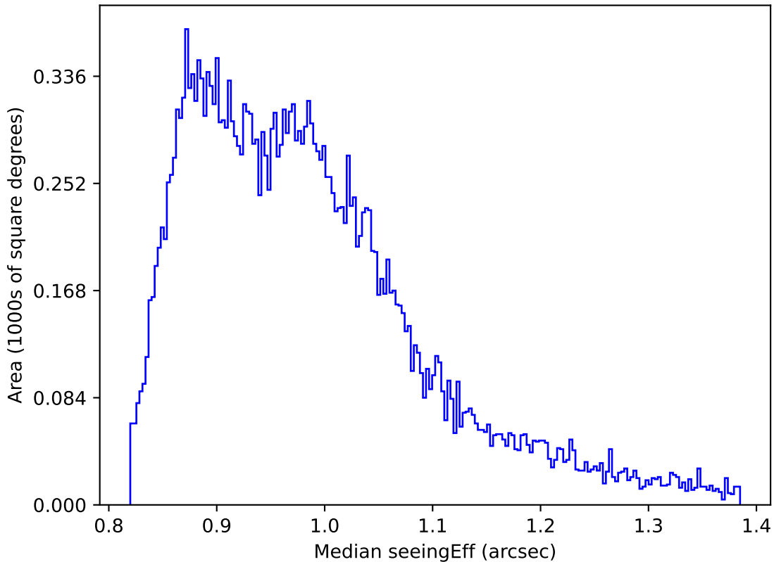
early_ss_template_fpextra2.0_v3.4_10yrs Yr 1 all bands: Median seeingEff
