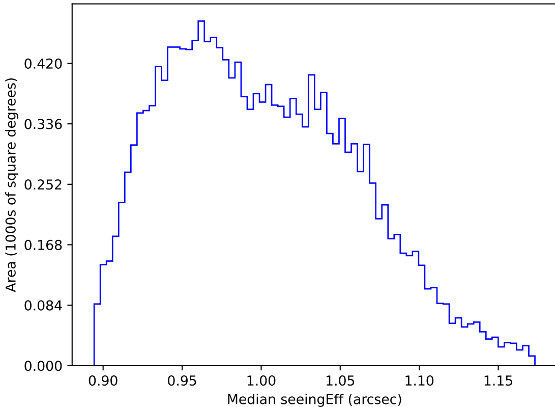
early_ss_template_fpextra2.0_v3.4_10yrs WFD y band: Median seeingEff
