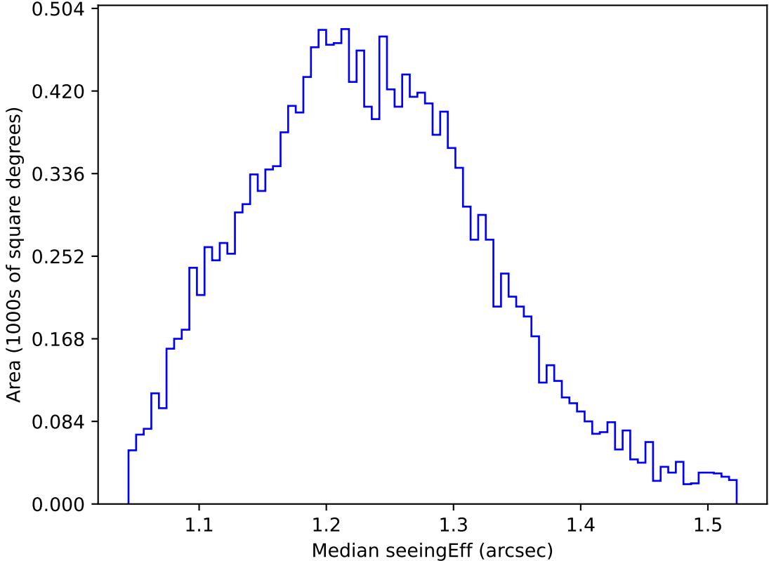
early_ss_template_fpextra2.0_v3.4_10yrs WFD u band: Median seeingEff
