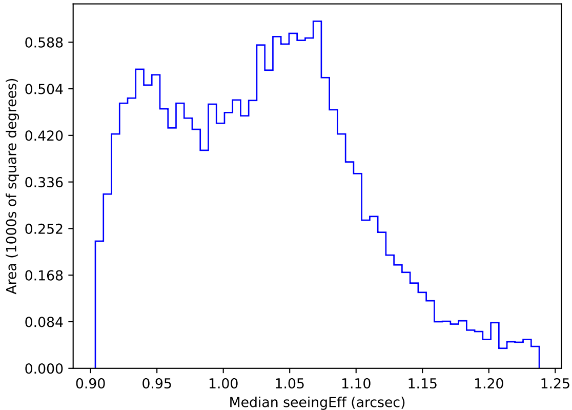
early_ss_template_fpextra2.0_v3.4_10yrs WFD all bands: Median seeingEff
