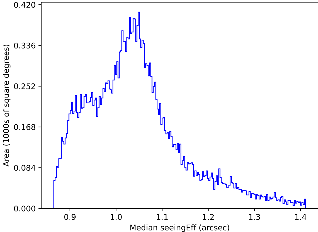
early_ss_template_fpextra2.0_v3.4_10yrs All sky z band: Median seeingEff
