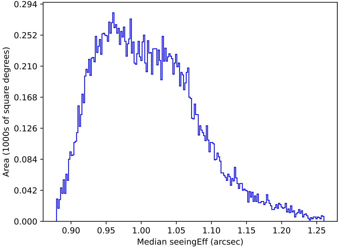
early_ss_template_fpextra2.0_v3.4_10yrs All sky y band: Median seeingEff
