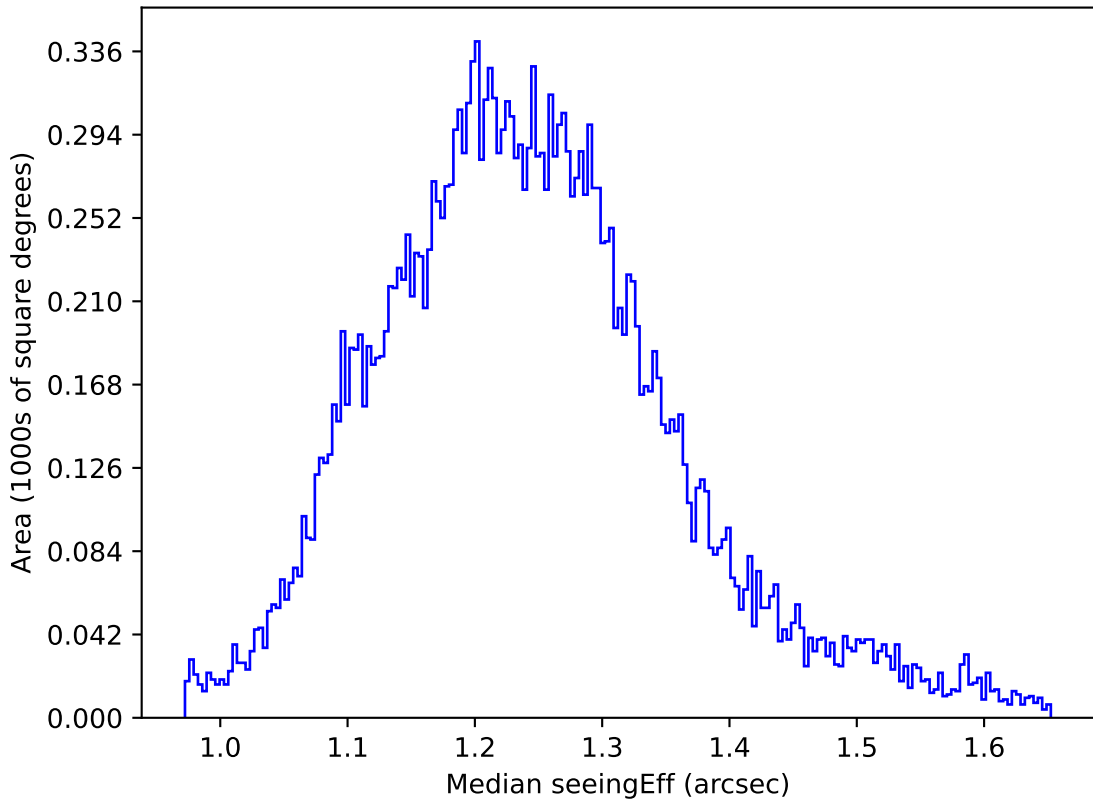
early_ss_template_fpextra2.0_v3.4_10yrs All sky u band: Median seeingEff
