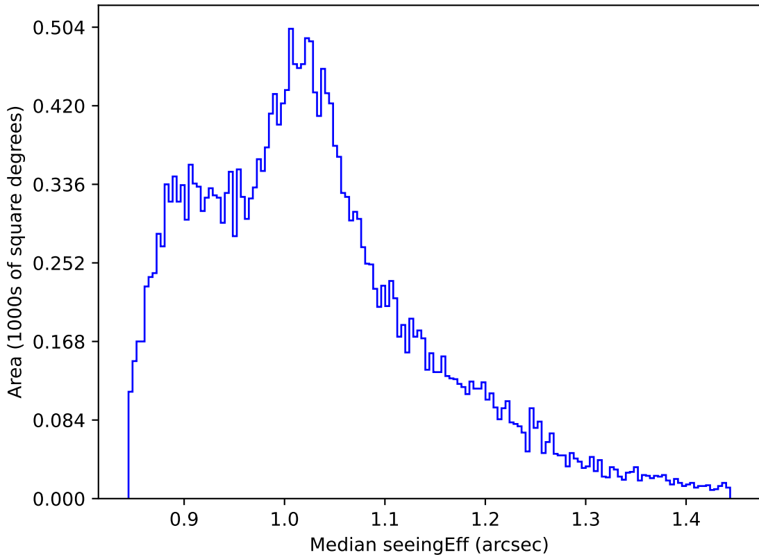
early_ss_template_fpextra2.0_v3.4_10yrs All sky i band: Median seeingEff
