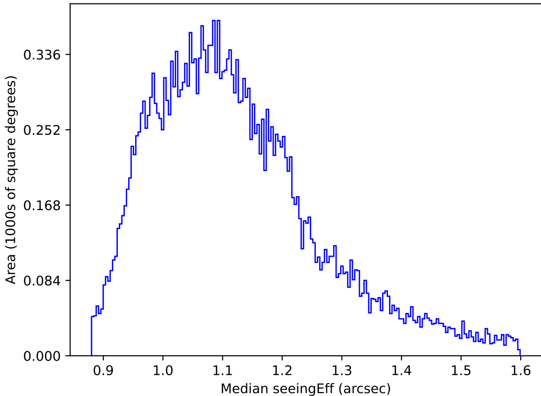
early_ss_template_fpextra2.0_v3.4_10yrs All sky g band: Median seeingEff
