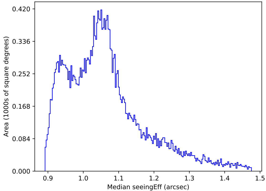
early_ss_template_fpextra2.0_v3.4_10yrs All sky all bands: Median seeingEff
