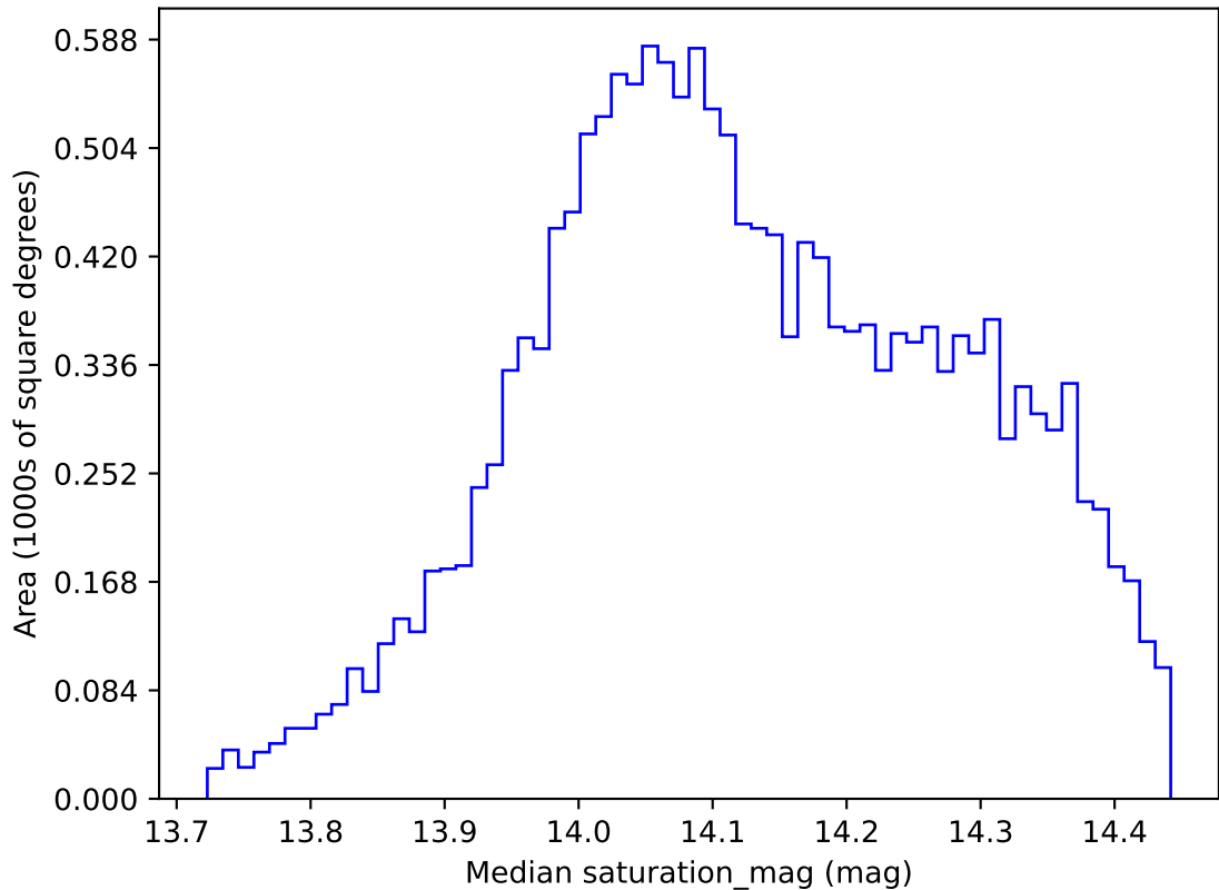
early_ss_template_fpextra2.0_v3.4_10yrs WFD z band: Median saturation_mag
