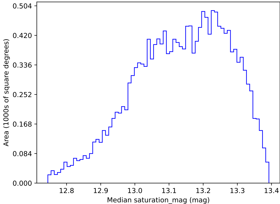
early_ss_template_fpextra2.0_v3.4_10yrs WFD y band: Median saturation_mag
