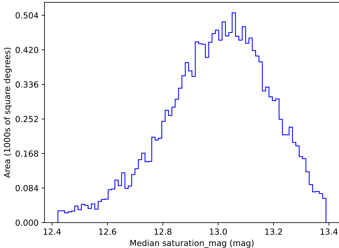
early_ss_template_fpextra2.0_v3.4_10yrs WFD u band: Median saturation_mag
