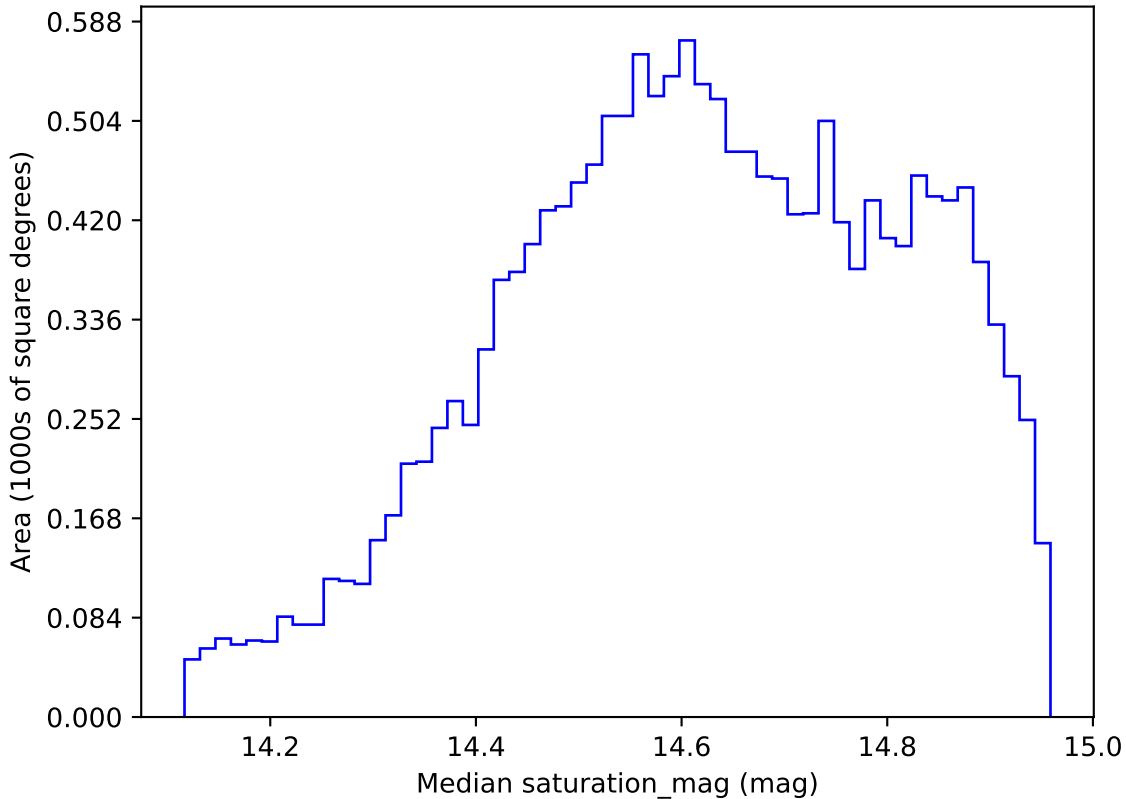
early_ss_template_fpextra2.0_v3.4_10yrs WFD r band: Median saturation_mag
