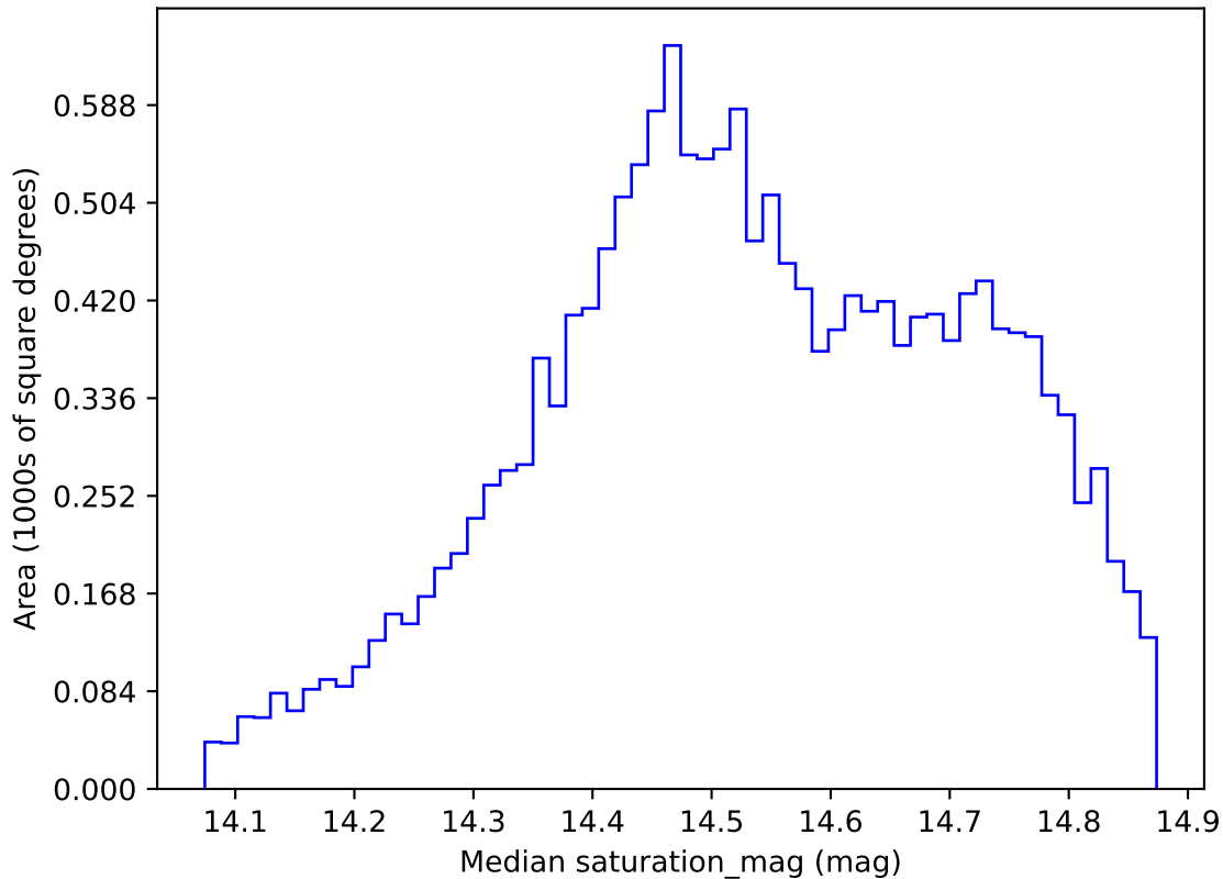
early_ss_template_fpextra2.0_v3.4_10yrs WFD i band: Median saturation_mag
