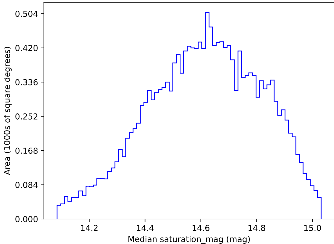
early_ss_template_fpextra2.0_v3.4_10yrs WFD g band: Median saturation_mag
