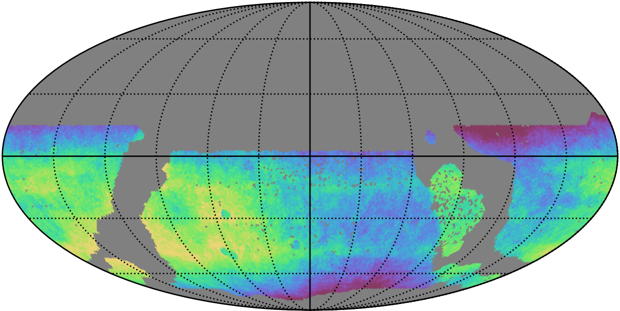
early_ss_template_fpextra2.0_v3.4_10yrs WFD all bands: Median saturation_mag
