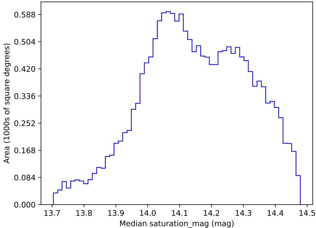
early_ss_template_fpextra2.0_v3.4_10yrs WFD all bands: Median saturation_mag
