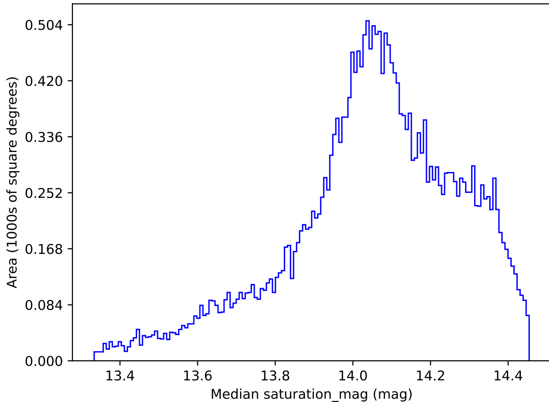
early_ss_template_fpextra2.0_v3.4_10yrs All sky z band: Median saturation_mag
