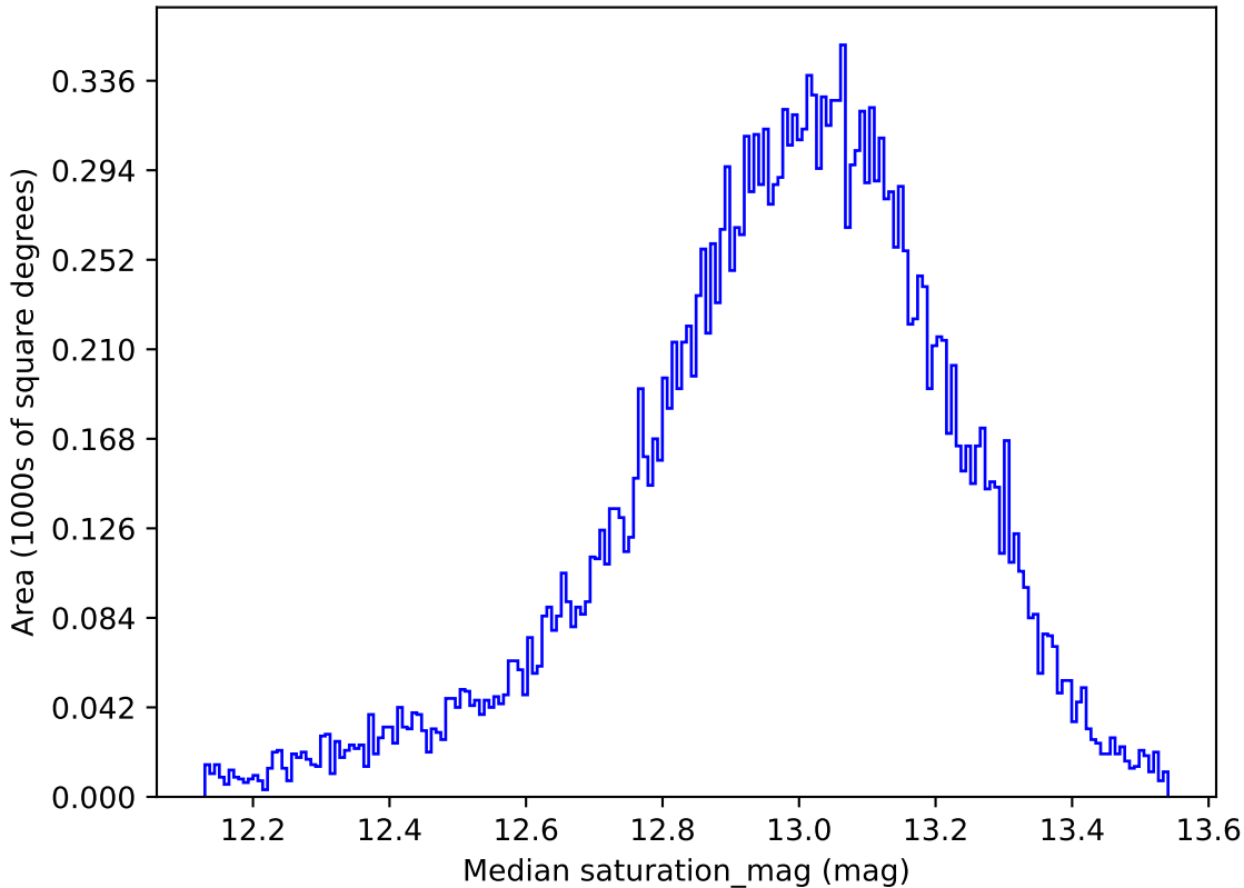
early_ss_template_fpextra2.0_v3.4_10yrs All sky u band: Median saturation_mag
