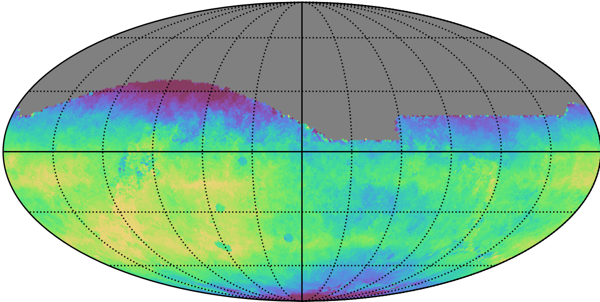
early_ss_template_fpextra2.0_v3.4_10yrs All sky r band: Median saturation_mag
