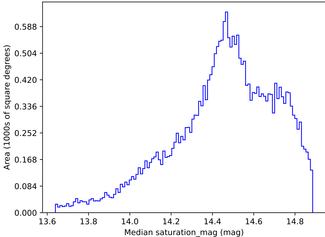
early_ss_template_fpextra2.0_v3.4_10yrs All sky i band: Median saturation_mag
