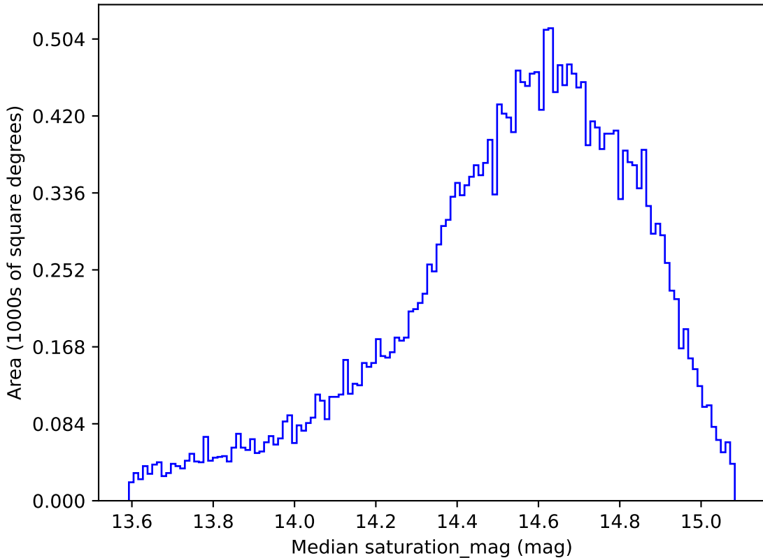
early_ss_template_fpextra2.0_v3.4_10yrs All sky g band: Median saturation_mag
